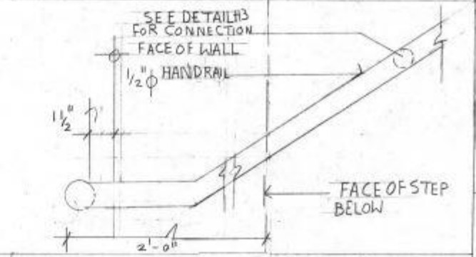
4 HANDRAIL TERMINATION SCALE: 3/8"=1'-0"
