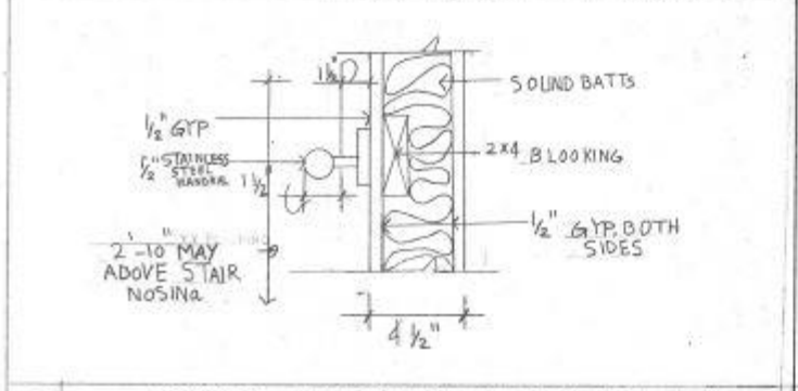
3 TYPICAL HANDRAIL @ 1-ALL SCALE: 3/8"=1'-0"
