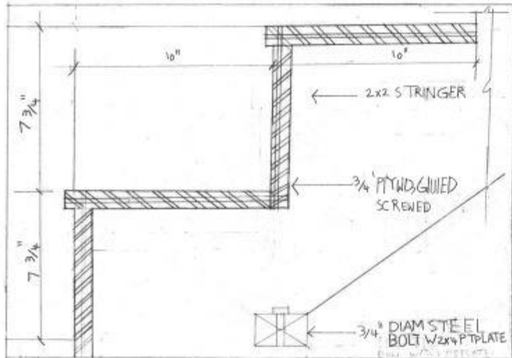
2 STRINGER TO FLOOR DETAIL SCALE: 3/8"=1'-0"
