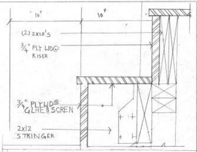
1 STRINGER TO LANDING DETAIL SCALE: 3/8"=1'-0"
